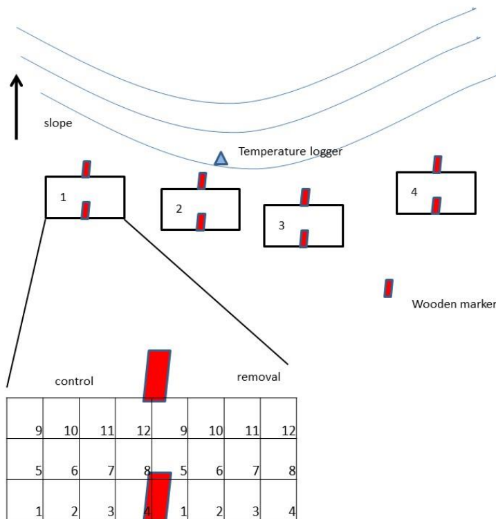
Figure 1. Setup of the pellet count plots and dwarf shrub recording plots within the snow bed design.
